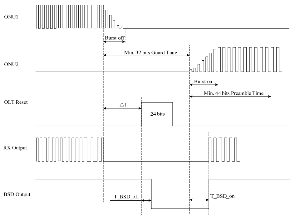
Figure 2 Reset Timing
